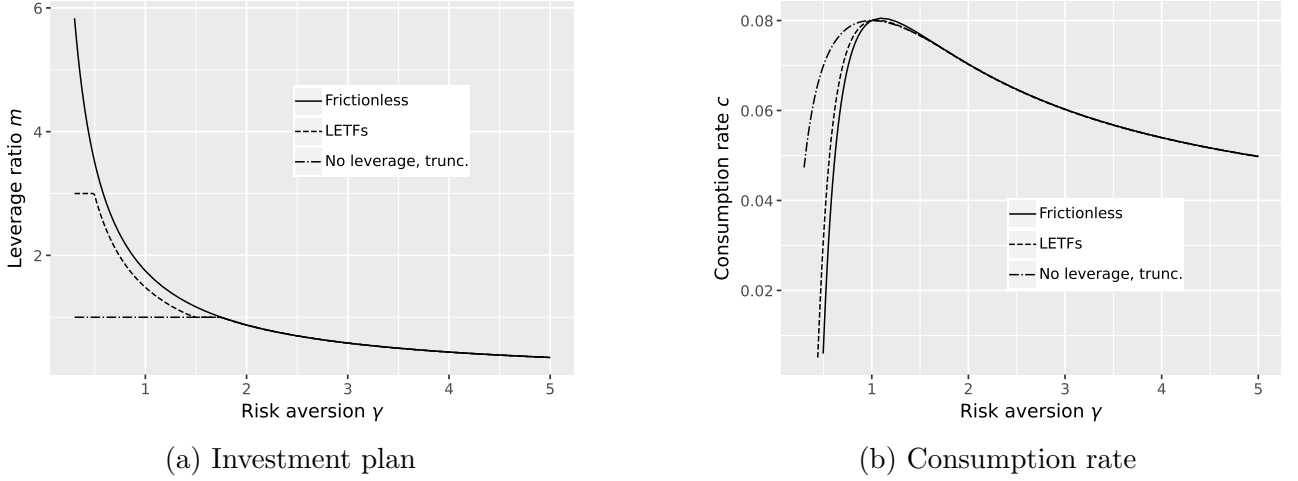
Figure 5: Solution comparison, infinite horizon
